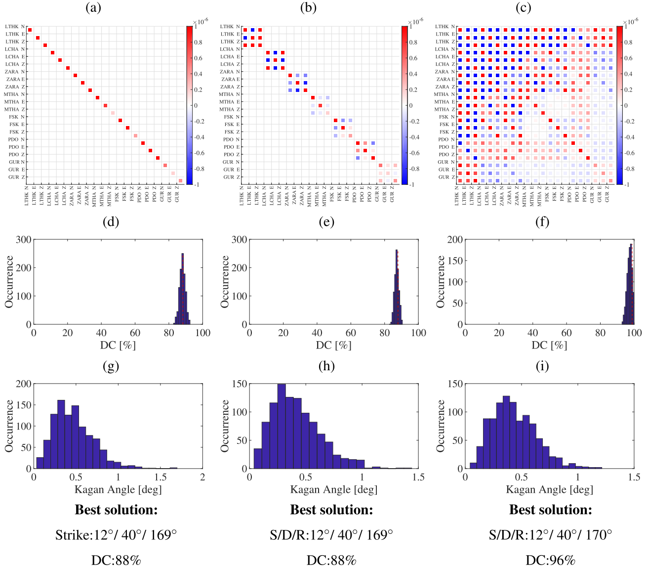
Figure 6. Coloured noise synthetic data tests for diagonal covariance matrix (a), block-diagonal covariance matrix (b), full covariance matrix (c), and the associated DC component (d)–(f), the related Kagan's angles (g)–(i) and maximum likelihood solutions (see the text).
